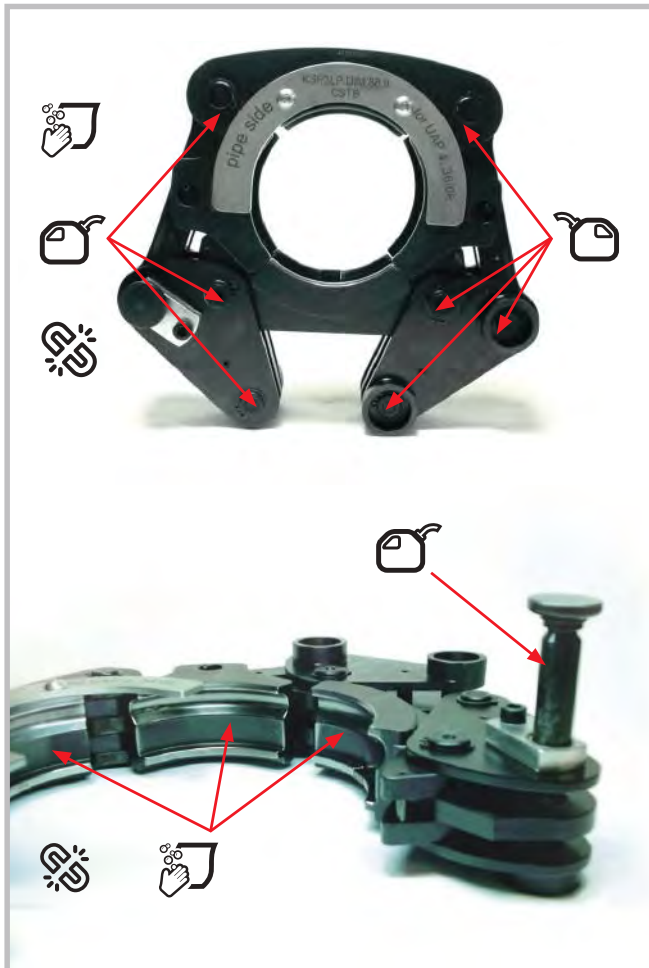
Figure 18 - Klauke equipment
